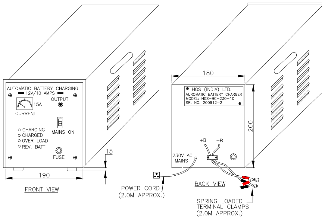
AUTOMATIC BATTERY CHARGER 12V TO 10AMPS
