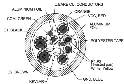
RESISTIVITY(ARS)CABLE with Bare Cond.
