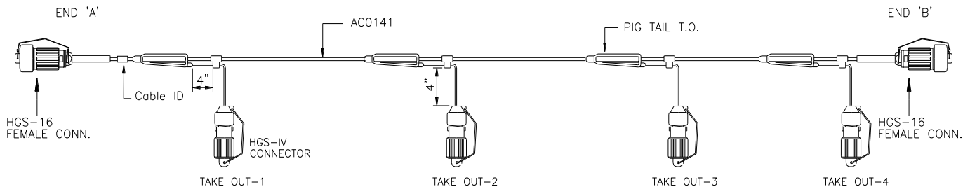
Aram/Aries Tri-Digital Land Cable with 4 take out
