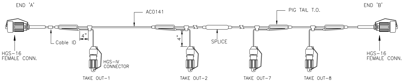
Aram/Aries Tri-Digital Land Cable with 8 take out
