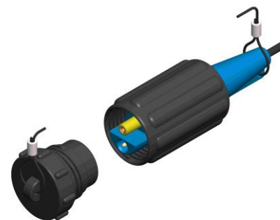
5515 Male screw fit connector
